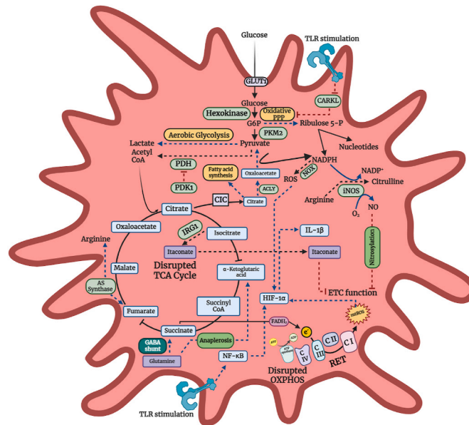
Fig. 9. Role of mtETC in M1 macrophage polarization. LPS, IFN- \gamma and/or TNF- \alpha (not shown here) stimulate reprogramming of macrophages toward the pro-inflammatory phenotype. During metabolic reprogramming, the TCA cycle is disrupted at two points (at the steps of \alpha -ketoglutarate and malate conversion) resulting in the accumulation of citrate and succinate, disrupting the feeding of electrons to the mtETC. The interruption activates the “Warburg effect” and shifts the cellular metabolism towards aerobic glycolysis to meet the energy demands. This results in the upregulation of glycolytic enzymes, and lactate production. M1 macrophages upregulate PKM2, catalyzing in the conversion of PEP into pyruvate and promoting glycolysis. Succinate synthesis is promoted in M1 macrophages via the channeling of glutamine into the TCA cycle through GABA shunt and through anaplerosis. Oxidation of succinate to fumarate via C II during low OXPHOS conditions results in the transfer of electrons in the opposite direction toward C I, leading to RET that induces mtROS production, which activates HIF-1 \alpha . HIF-1 \alpha , a signaling molecule characteristic of the M1 phenotype, drives the production of pro-inflammatory cytokines, such as IL-1 \beta . In M1 macrophages, oxidation of G6P is enhanced due to an increase in oxidative PPP which generates NADPH that is required for NOX-induced ROS (shown by broken black arrow), synthesis of fatty acids, and anti-oxidant defense mechanisms, and ribulose-5P that is required for nucleotide biosynthesis, and this occurs due to suppressed activity of CARLK. M1 macrophages show upregulation in the PDK1 enzyme, a regulatory enzyme that phosphorylates PDH that catalyses the conversion of pyruvate to acetyl coA. Pyruvate-derived acetyl CoA (shown by broken black arrow) enters into the TCA cycle that generates NADH which fuels mtETC. Reduction in IDH1 levels led to an increase in the synthesis of antimicrobial molecule i.e., itaconic acid (or Itaconate) via IRG1 from decarboxylation of aconitate. However, increased production of itaconate inhibits SDH activity. Furthermore, citrate is exported from the mitochondria via CIC, and broken down into oxaloacetate and acetyl CoA via ACLY. Acetyl CoA can be used as a substrate for fatty acid synthesis. Oxaloacetate is metabolized to pyruvate accompanied by NADPH and NO production. In M1 macrophages, iNOS activity is upregulated, resulting in the catabolism of arginine to citrulline and NO (shown by broken black arrow), the latter playing a crucial antimicrobial role in M1 macrophages. Citrulline is metabolized along with aspartate to generate argininosuccinate via ASS, which is further catalyzed into arginine and fumarate. Further, NO-induced nitrosylation of Fe-S proteins in C I, and C IV results in their inactivation resulting in low OXPHOS. The black solid arrows represent the movement of substrates, the broken blue arrows represent the activation of enzymatic and signaling pathways in M1 macrophages, and the broken red line represent the inhibition of the enzymes/pathways in M1 macrophages. Abbreviations used are: GLUT1, glucose transporter 1; CARLK, carbohydrate kinase-like protein; PPP, pentose phosphate pathway; G6P, glucose-6-phosphate; PKM2, pyruvate kinase M2; PDH, pyruvate dehydrogenase; PDK1, pyruvate dehydrogenase kinase 1; CIC, citrate carrier; IRG1, immune responsive gene 1; ASS, argininosuccinate synthase; GABA, \gamma -amino butyric acid; NOX, NADPH oxidase; mtROS, mitochondrial ROS; CIC, citrate carrier; ACLY, ATP-citrate lyase; NO, nitric oxide; iNOS, inducible NO synthase; ASS, argininosuccinate synthase; RET, reverse electron transfer; PEP, phosphoenolpyruvate. (For interpretation of the references to colour in this figure legend, the reader is referred to the Web version of this article.)
