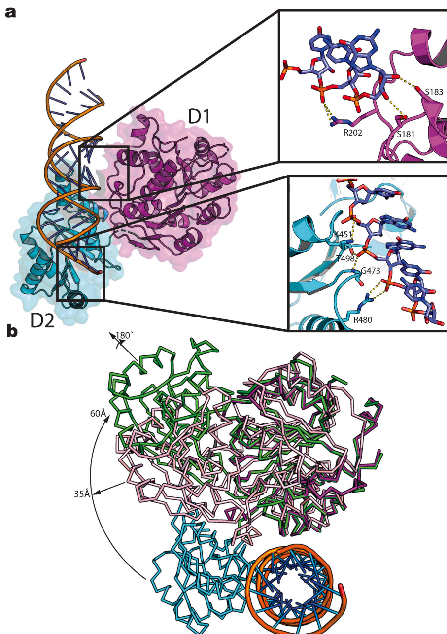
Fig. 2. The structure of DDX3X bound to duplex RNA. (a) The two RNA binding domains (D1 in purple and D2 in cyan) are in ribbon representation, overlapped with their surface representation, whereas the RNA in ribbon representation is in orange with the bases coloured in purple. The insets show the hydrogen bonds network between both the phosphates backbone and the oxygen atoms of the nucleotides of the RNA and the side chains of the protein. (b) Conformational changes between the apo-DDX3X (PDBid:5E7I), DDX3X in complex with the double stranded RNA (PDBid:5E7I) and VASA (PDBid:2DB3) structures. The structural alignment was performed by C- \alpha superposition. Structures superposition was performed with Coot (Emsley et al., 2010). The figure was prepared with PyMOL ( http://www.pymol.org/ ). (For interpretation of the references to colour in this figure legend, the reader is referred to the Web version of this article.)
