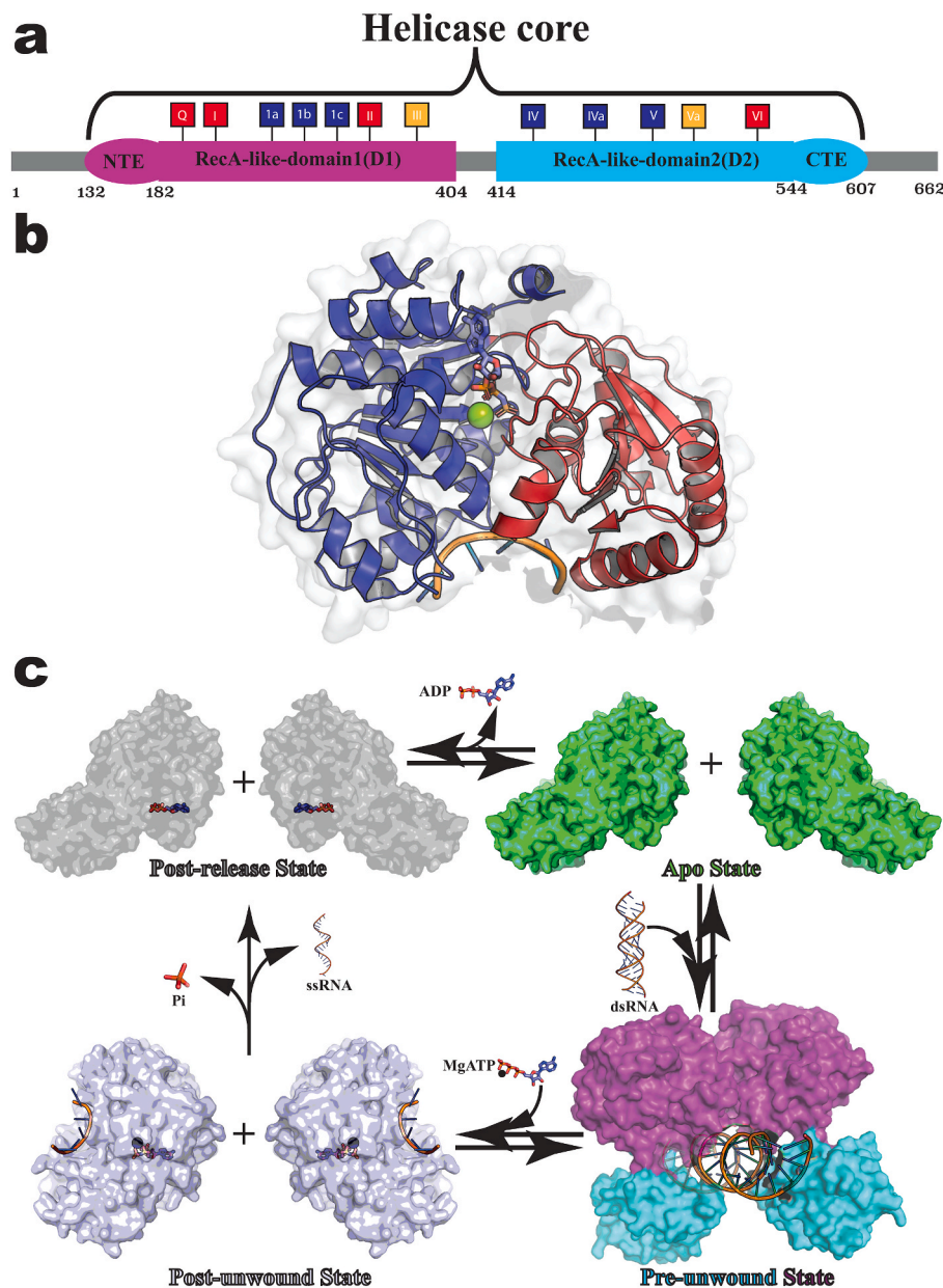
Fig. 1. Protein domains organization and conserved motifs of DDX3X RNA helicase. (a) The catalytic helicase core is composed of two RecA-like domains, domain 1 (encompassing helicase motifs Q, I, II, III) and domain 2 (encompassing helicase motifs IV, V and VI). These domains are essential for RNA binding and ATPase activity.
