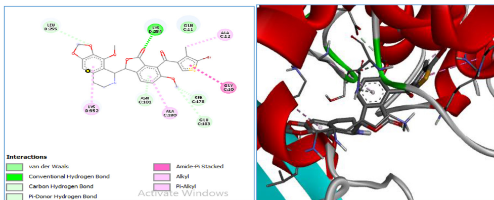
Figure 9: 2-D and 3-D visualization of compound D4 in the active pocket of the receptor.
