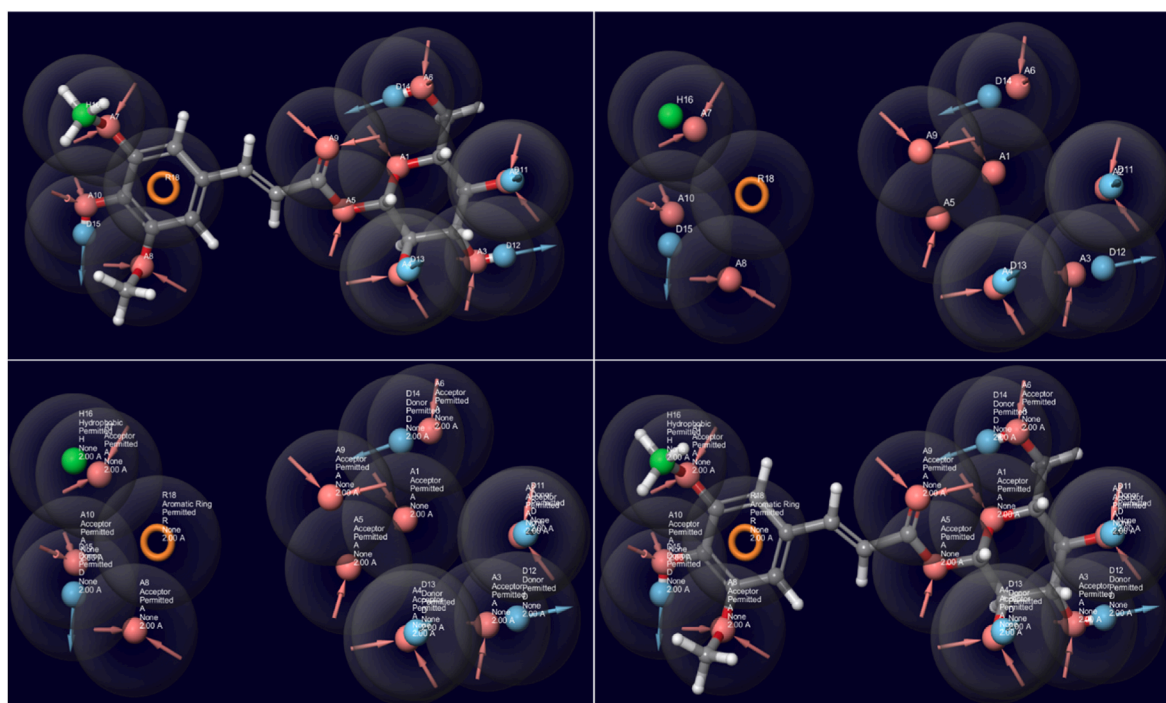
Fig. 4. Pharmacophore hypothesis of 1-O- \beta -D-glucopyranosyl sinaoate. (Orange color: HB Acceptor, Blue color: HB Donor; Green color: Hydrophobic; Yellow color: Aromatic ring). (For interpretation of the references to color in this figure legend, the reader is referred to the Web version of this article.)
