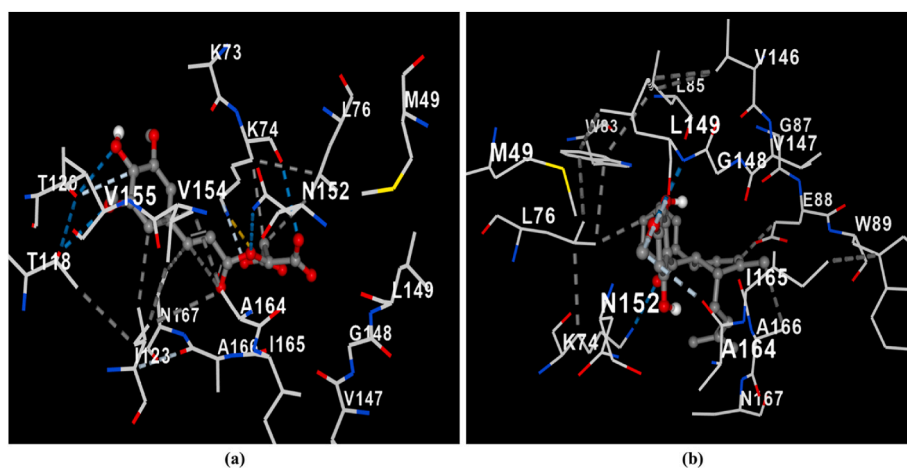
Fig. 3. Binding affinities among the residues of non-structural protein (PDB ID: 2FOM) of DENV-2 with (a) Sinapoyl malate and (b) Panduratin A. (Dash line showed the bound) (Blue color: hydrogen bonds; Sky blue color: weak hydrogen bonds; Black color: Hydrophobic interactions; Yellow color: ionic interactions). (For interpretation of the references to color in this figure legend, the reader is referred to the Web version of this article.)
