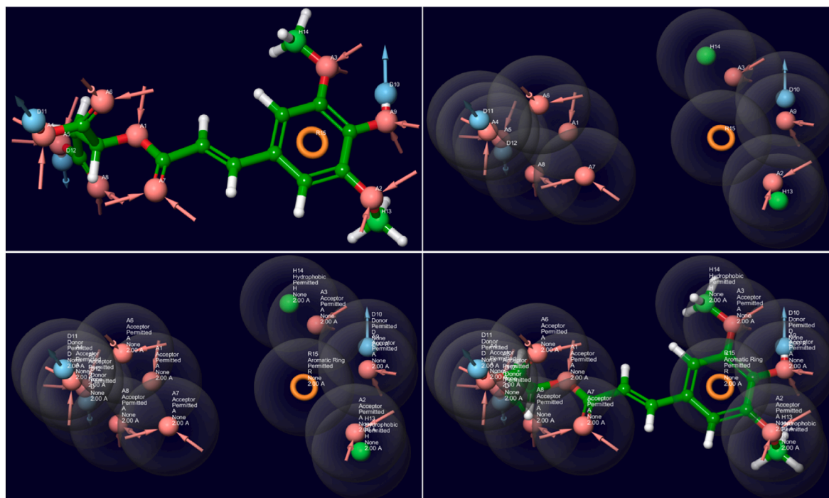
Fig. 5. Pharmacophore hypothesis of Sinapoyl malate. (Orange color: HB Acceptor, Blue color: HB Donor; Green color: Hydrophobic; Yellow color: Aromatic ring). (For interpretation of the references to color in this figure legend, the reader is referred to the Web version of this article.)
