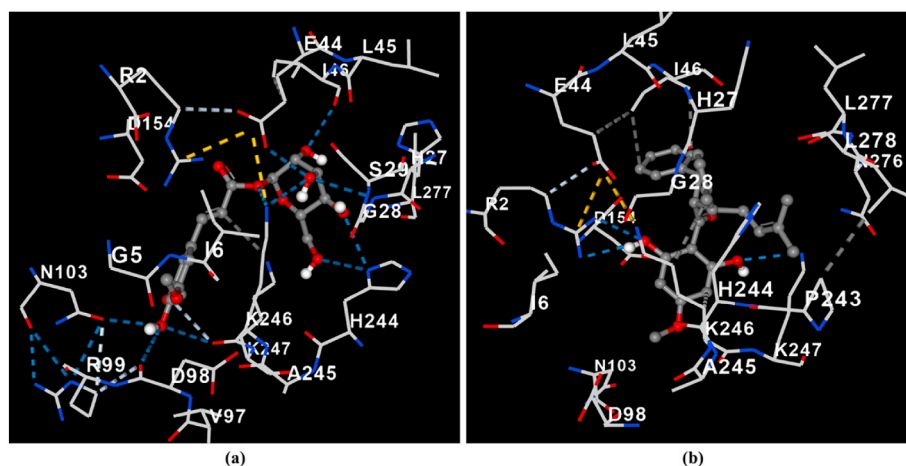
Fig. 2. Binding affinities among the residues of structural protein (PDB ID: 1OKE) of DENV-2 with (a) 1- O - \beta -D-Glucopyranosyl sinaoate and (b) Panduratin A. (Dash line showed the bound) (Blue color: hydrogen bonds; Sky blue color: weak hydrogen bonds color; Black: Hydrophobic interactions; Yellow color: ionic interactions). (For interpretation of the references to color in this figure legend, the reader is referred to the Web version of this article.)
