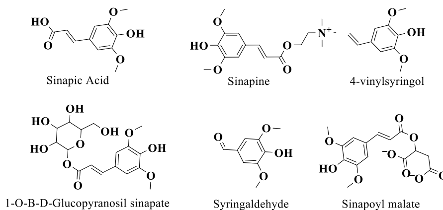
Fig. 1. SA and its derivatives.
