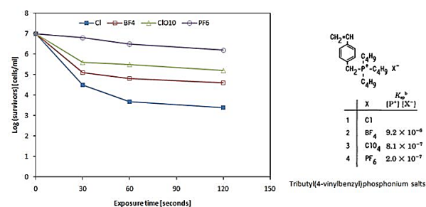
Figure 10. Effect of counterion composition to antimicrobial activity for tributyl(4-vinylbenzyl) phosphonium salts at 2.8 mM against S. aureus , and its relationship with solubility product constant of polymer KSP. 61
