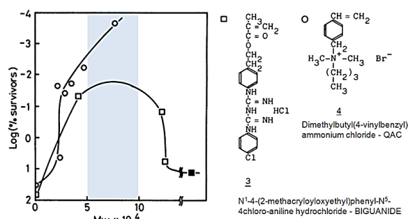
Figure 4. Effect of MW on antibacterial activity against S. aureus . □ poly 3, 23 \mu\text{M} ; ○ poly 4, 2.0 \mu\text{M} ; ■ plot for microgel of poly 3. 60
