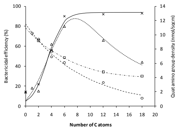
Figure 14. Bactericidal efficiency ( \Delta × = alkylated-PEI, × = alkylated-methylated-PEI) against S. aureus and density of quaternary ammonium group (○ = alkylated-PEI, □ = alkylated-methylated-PEI) of PEI immobilized on the glass. From Table.
