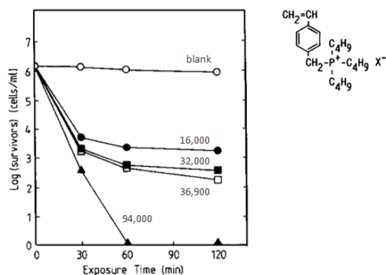
Figure 5. Plots of log (survivors) versus exposure time of S. aureus to tributyl(4-vinylbenzyl) phosphonium chloride (2.8 \mu\text{M} ) of various MW: ○ blank; \Delta 94,000; □ 36,900; ■ 32,000; ● 16,000. X = Cl.
