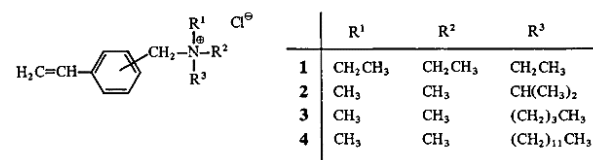
Figure 3. Poly [trialkyl (vinylbenzyl) ammonium chloride]. 58,59
