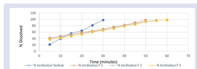
Figure 3. Dissolution Curve of Paracetamol Microcapsules for Each Formula.
