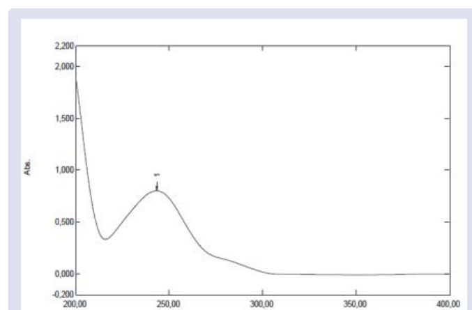
Figure 1. Maximum Absorption Wavelength of Paracetamol ( \lambda = 244.2 nm).
