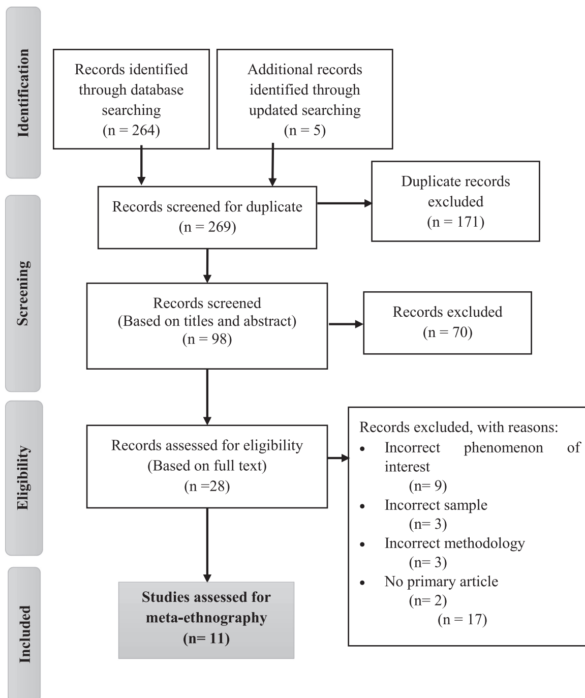
Fig. 1. PRISMA flowchart.
